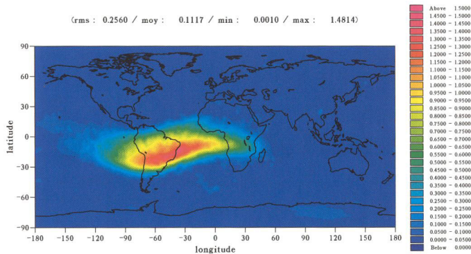
Fig. 7 Plot of the relative SAA dose exposure in 2002–2005 at the 1,300 km altitude of Jason-1 (dimensionless units)
