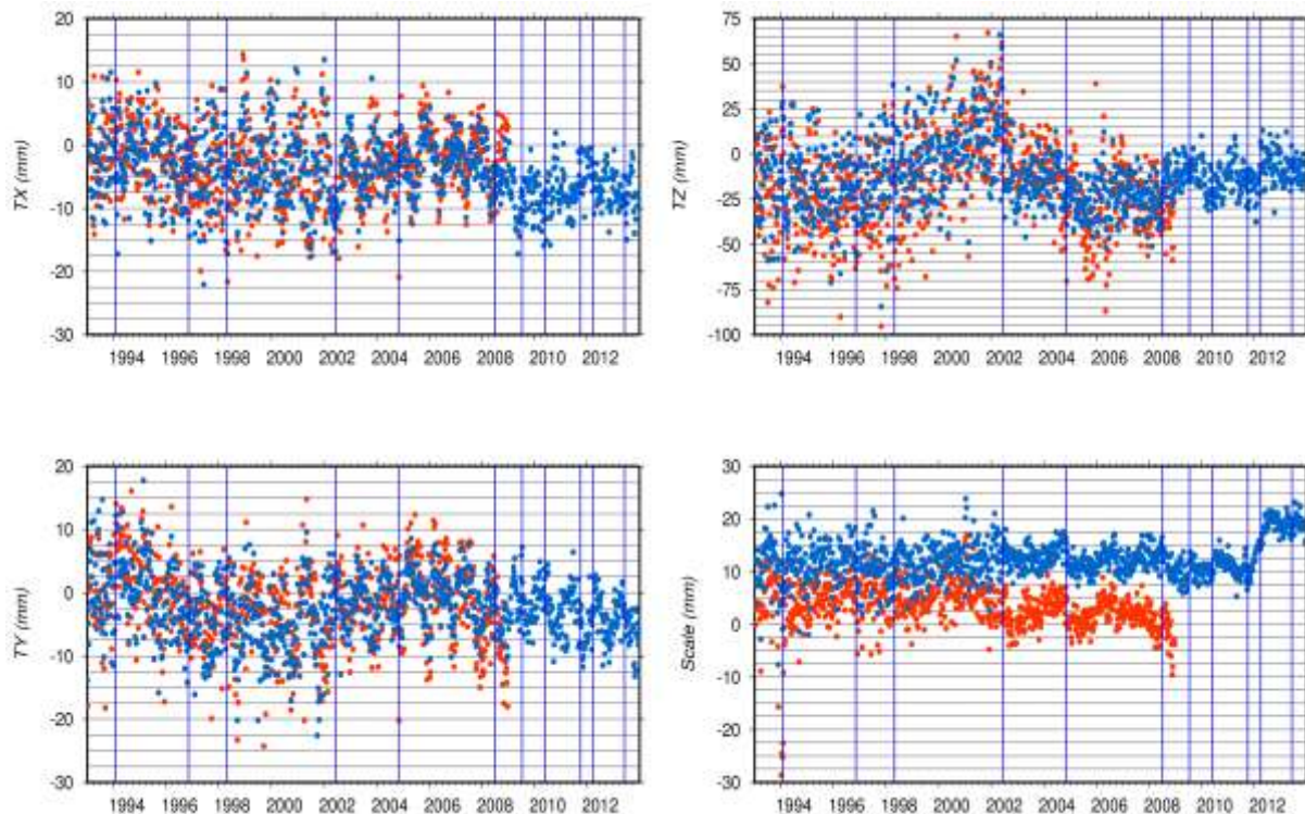
Figure 1 - Helmert parameters (translations and scale of the IDS contributions to ITRF2008 (red) and ITRF2013 (blue) with respect to ITRF2008.
