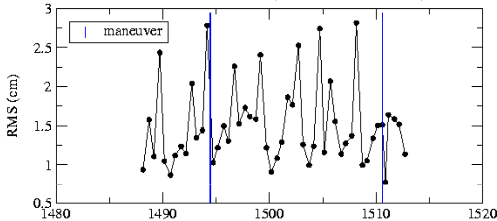
SLR Jason2
