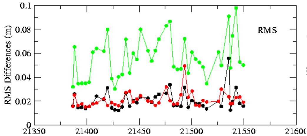
Jason2 Rad/Crs/Alg Orbit Differences for LCA vs CNES_POD from July_2008 to January_2009
