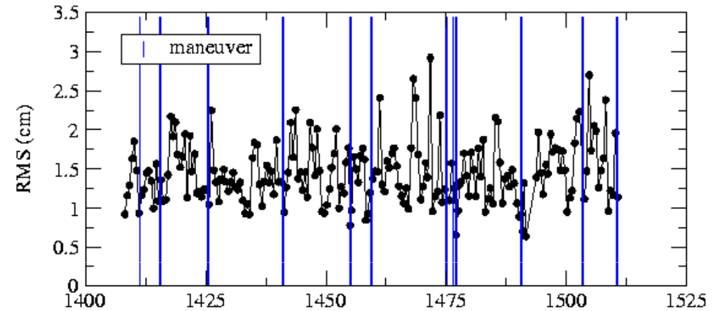
SLR Jason1
