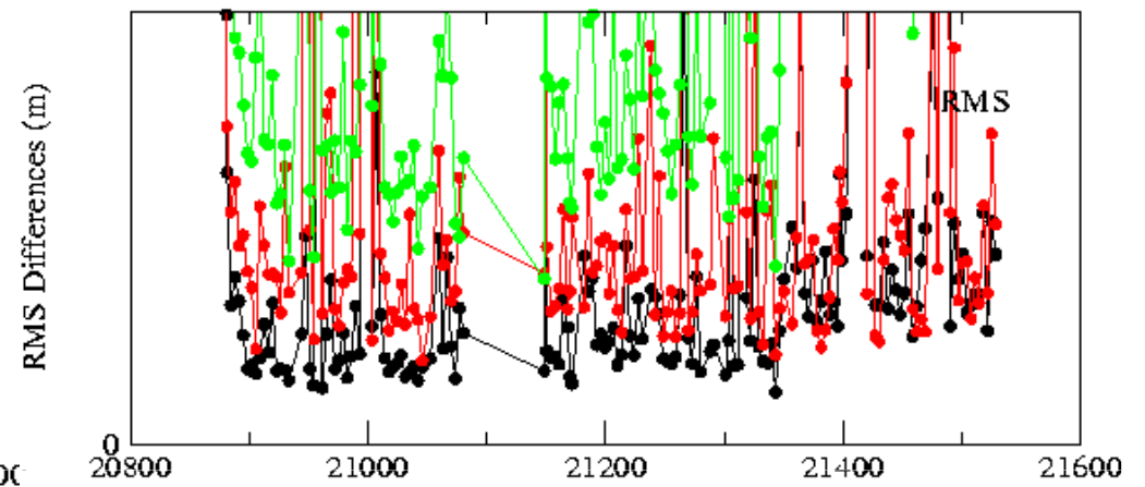
Jason1 Rad/Crs/Alg Orbit Differences for LCA vs CNES_POD from 03/2007 to 12/2008
