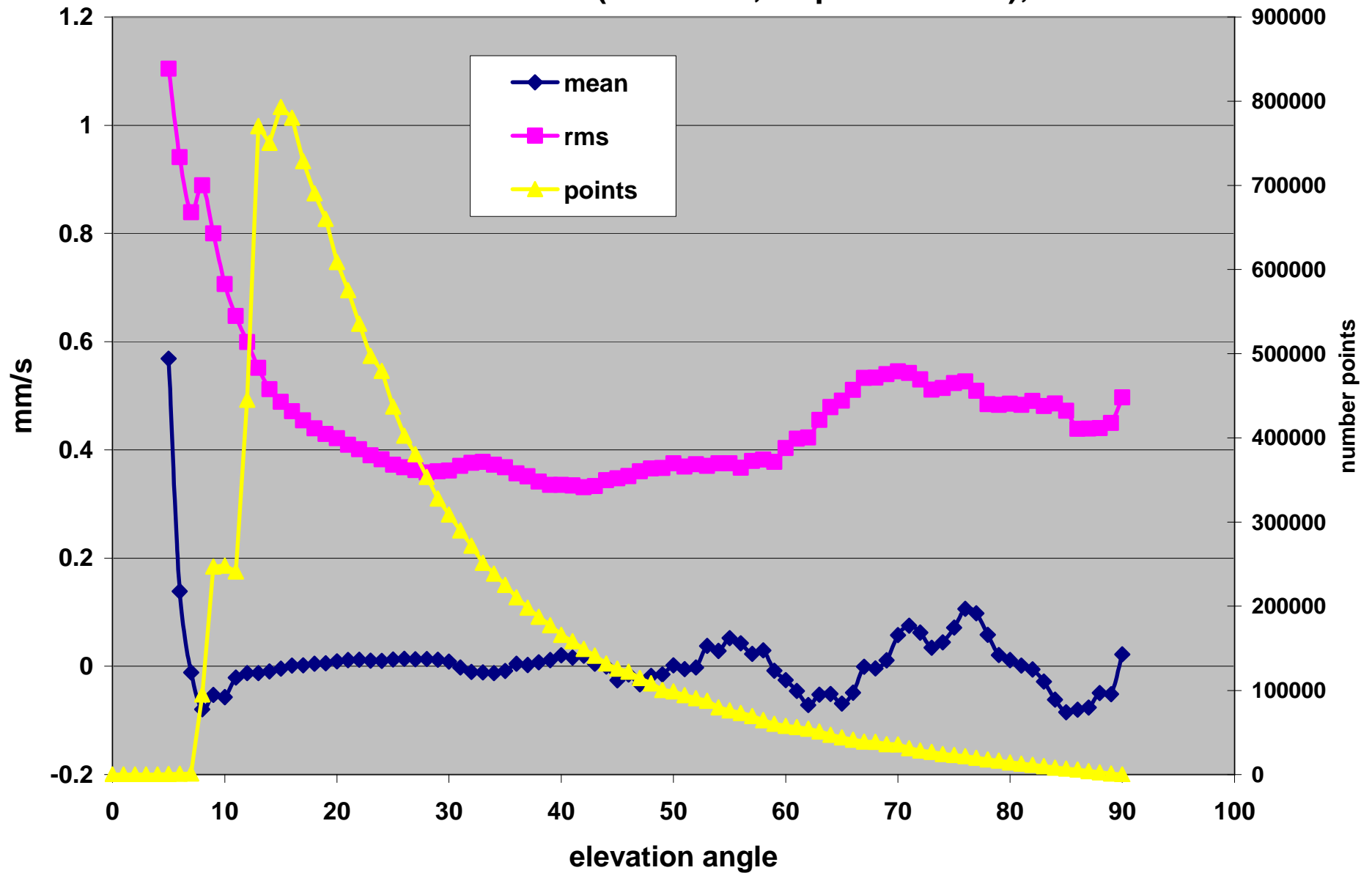
SPOT5 DORIS residuals (ITRF2005, Hopfield model); 2003-2007
