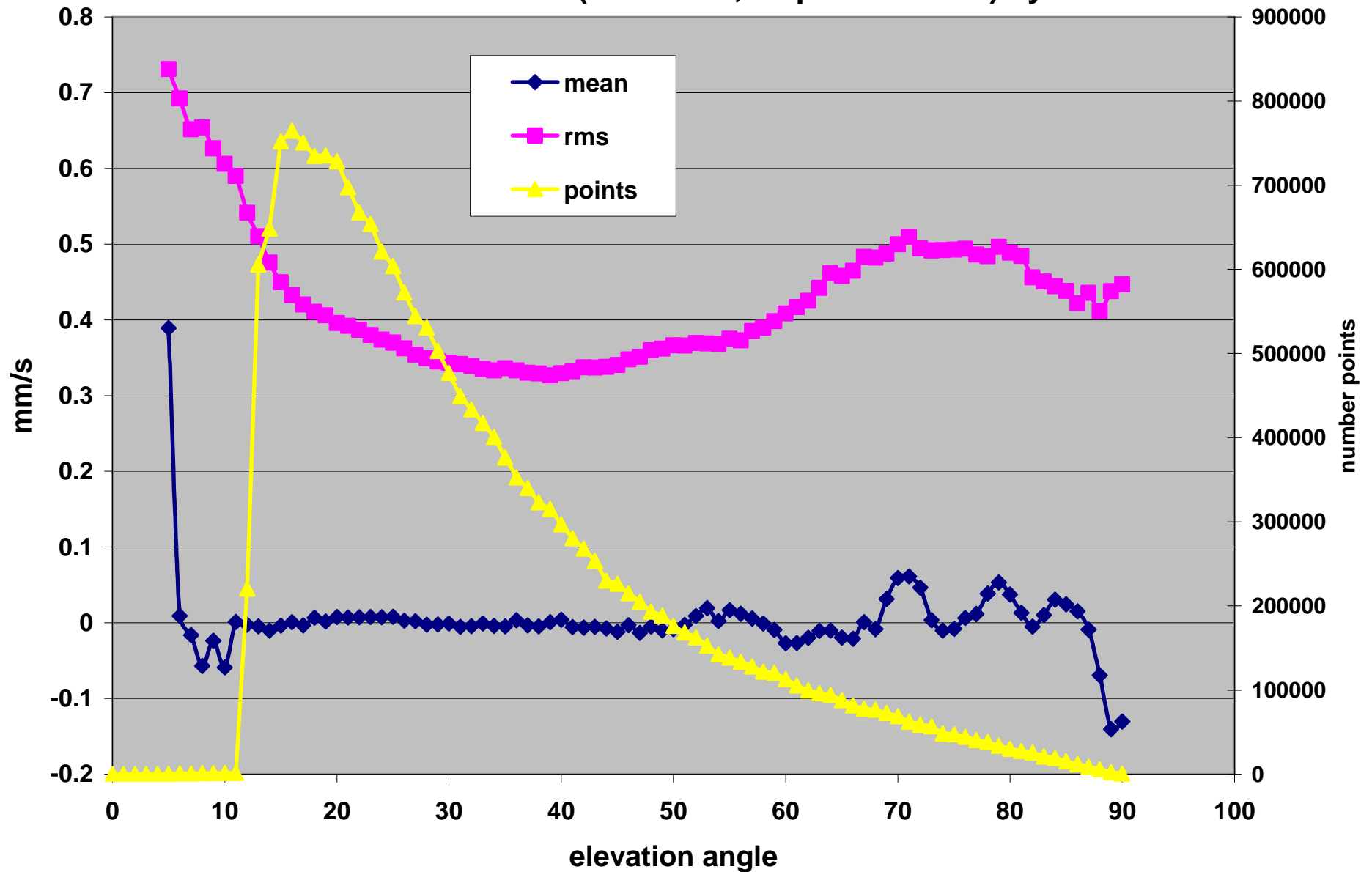
Jason DORIS residuals (ITRF2005, Hopfield model) cycles 1-186
