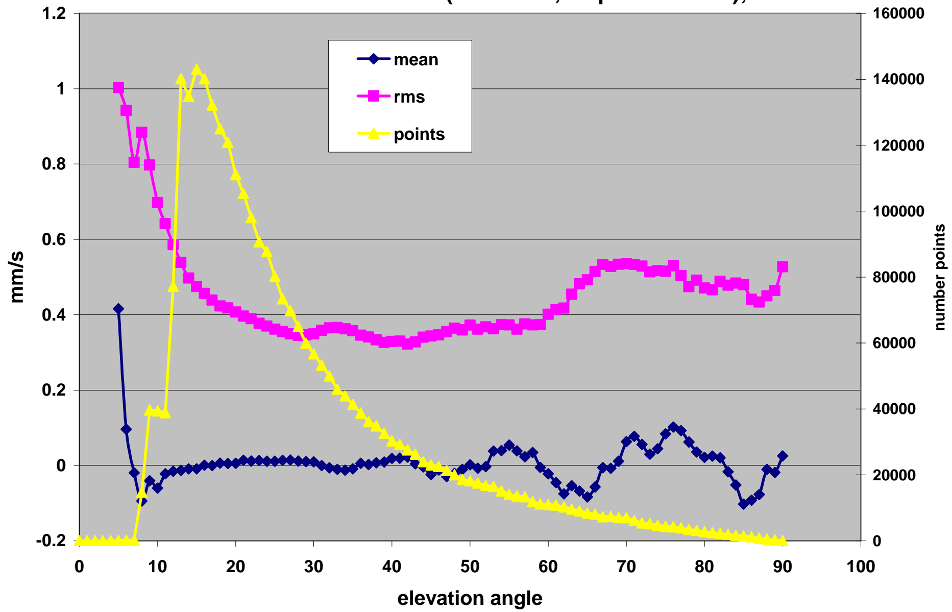
SPOT5 DORIS residuals (ITRF2005, Hopfield model); 2005
