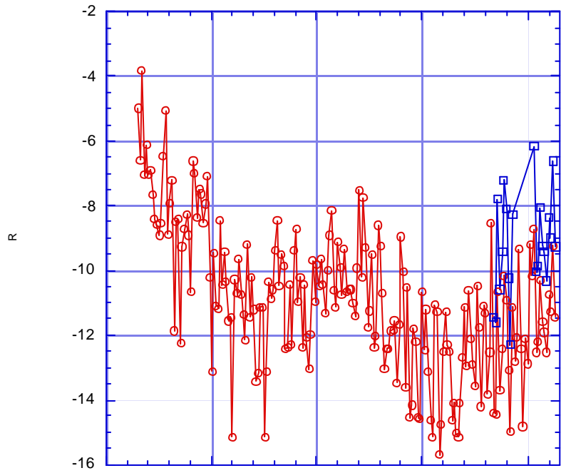
R_OFF_021114.kl
