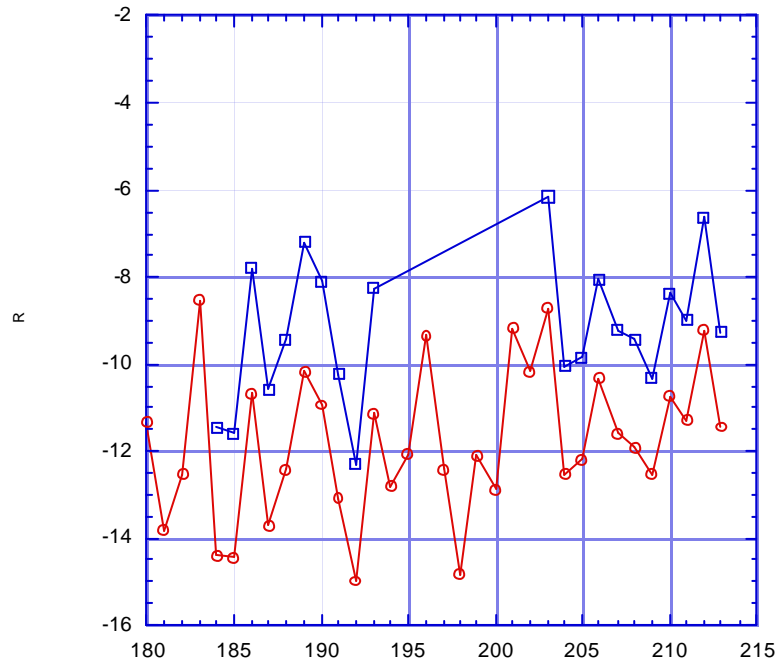
R_OFF_021114.kl
