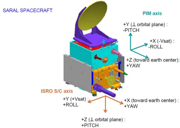
Figure 8 Schematic view of SARAL satellite
