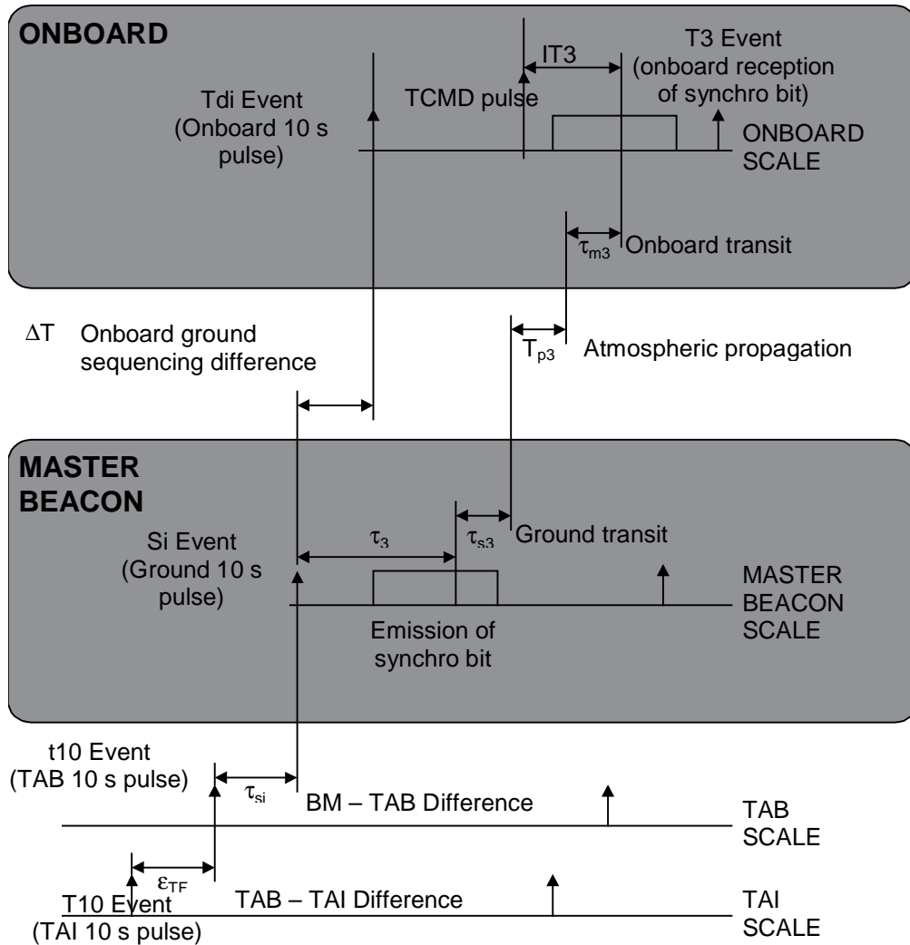
Figure 1 : Diagram showing the time-tagging measurement principle (TAB = TAC or TAK)
