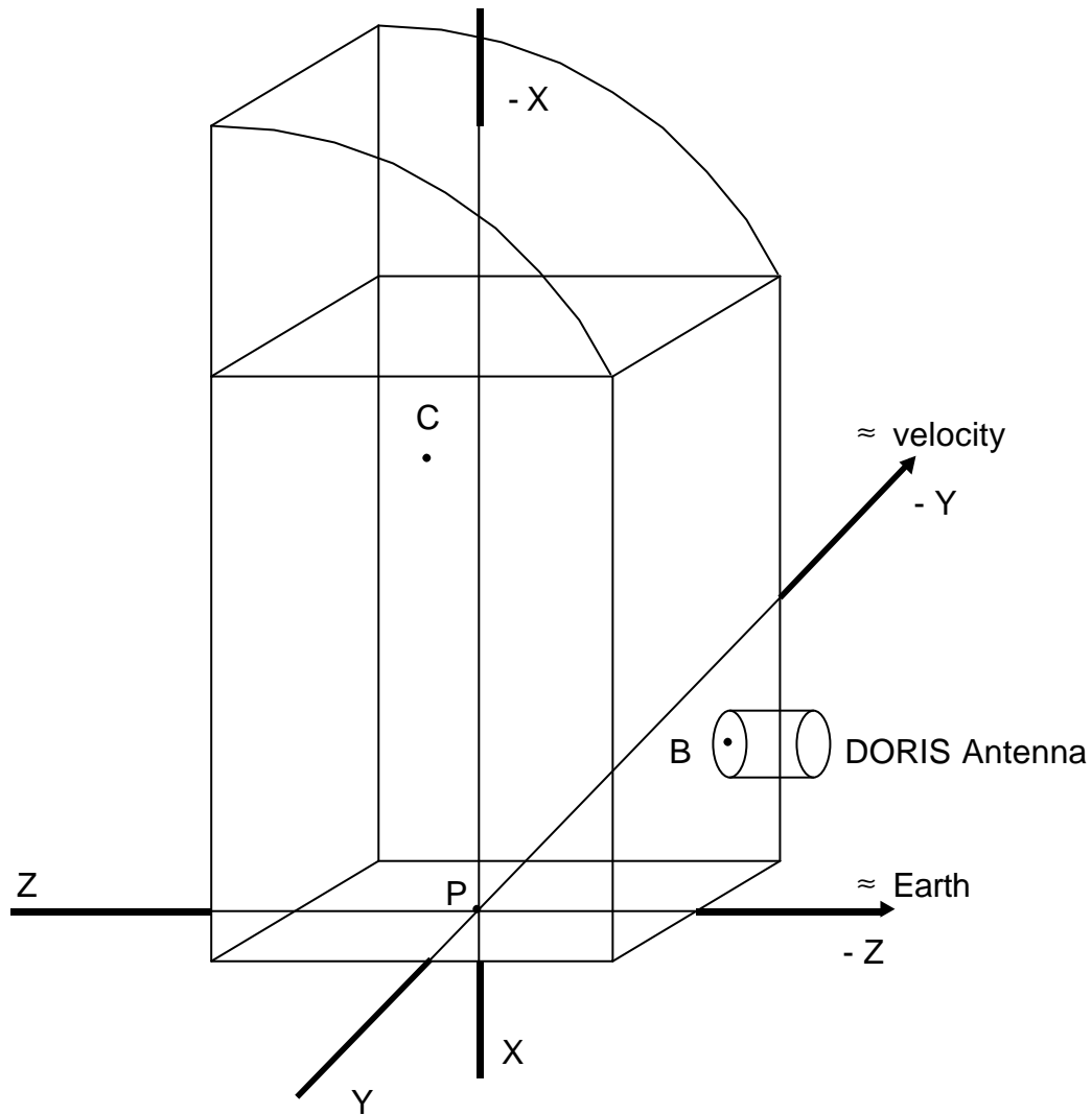
Figure 4 : Position of DORIS antenna on the SPOT5 satellite
